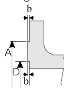
Type G 'O' Ring recess
