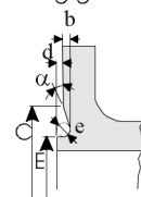
Type H 'O' Ring groove
